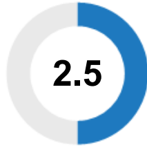
Overall Score
